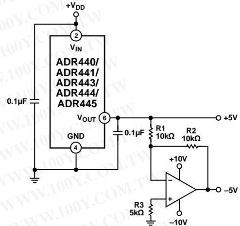
Figure 36. ADR44x Bipolar Outputs
