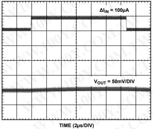
Figure 9. Output Response to 100 \mu A Input Current Change with 1 \mu F Capacitor
