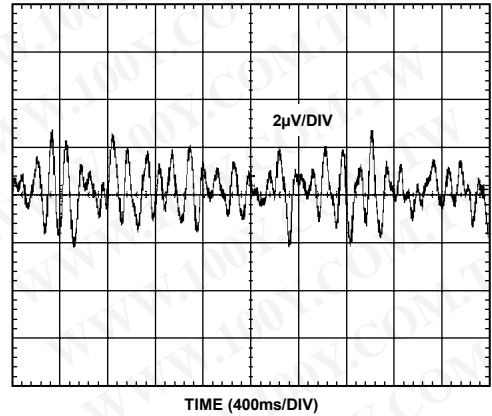
Figure 10. 1 Hz to 10 Hz Noise
