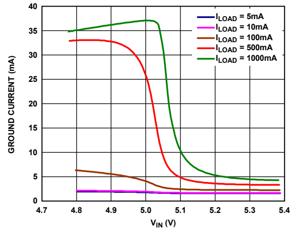
Figure 13. Ground Current vs. Input Voltage ( V_{IN} ) in Dropout, V_{OUT} = 5\text{ V}
