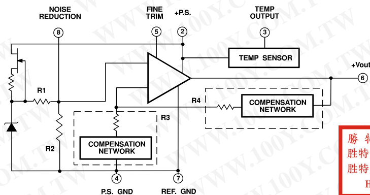
Figure 1. BLOCK DIAGRAM
