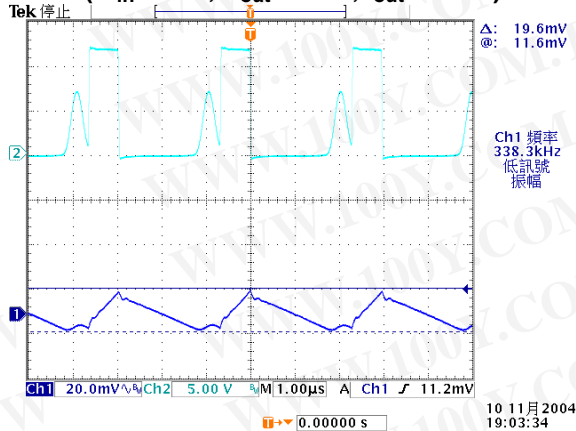
AP1520 Vout Ripple ( V_{in} = 12V ; V_{out} = 3.3V ; I_{out} = 0.1A )
