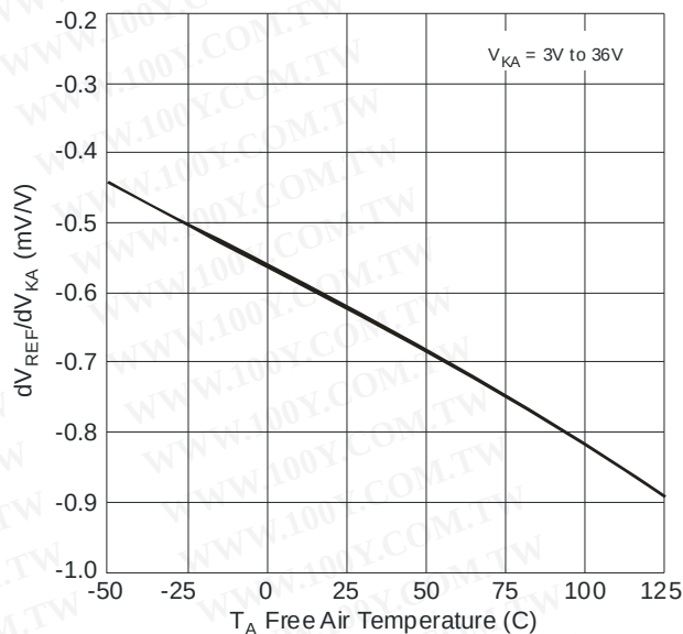
Ratio of Delta Reference Voltage to Delta Cathode Voltage vs. Free Air Temperature
