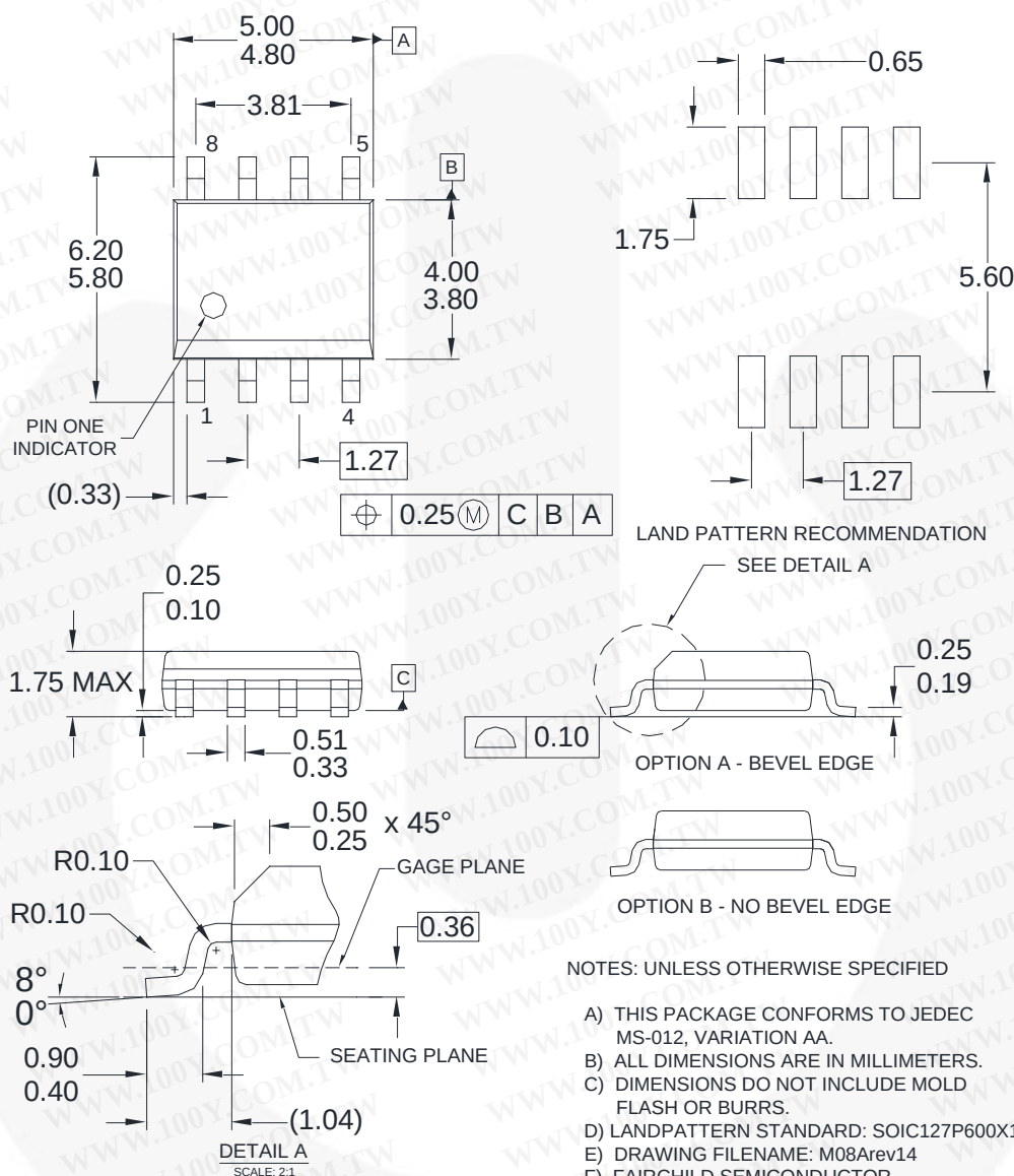
Figure 32. 8-Pin, SOP-8 Package
