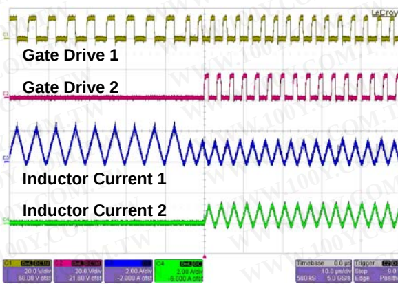
Figure 48. Phase-Adding Operation
