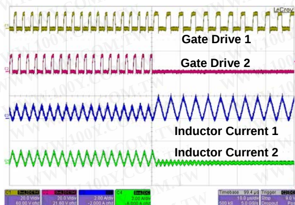
Figure 47. Phase-Dropping Operation
