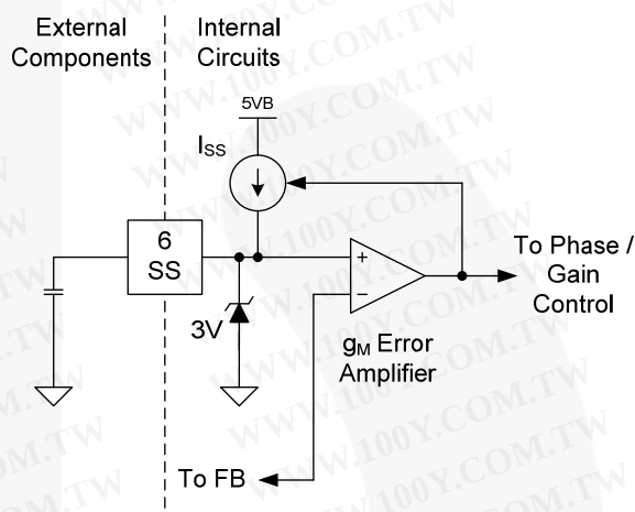
Figure 19. Soft-Start Programming
