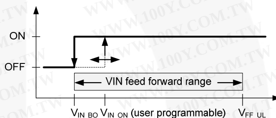
Figure 30. VIN Turn-on and Turn-off Thresholds
