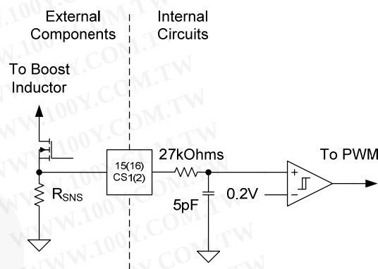
Figure 26. Current-Sense Protection Circuits
