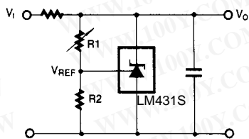
Figure 13. Shunt Regulator
