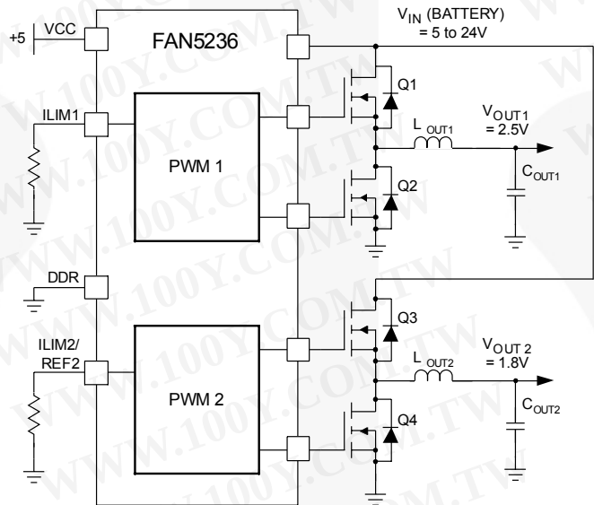
Figure 1. Dual-Output Regulator
