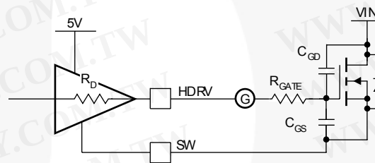
Figure 18. Drive Equivalent Circuit
