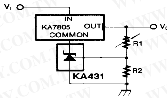
Figure 12. Output Control for Three-Terminal Fixed Regulator
