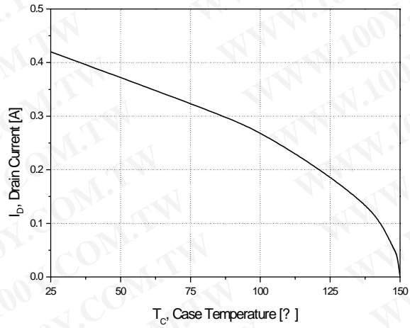
Figure 10. Max. Drain Current vs. Case Temperature
