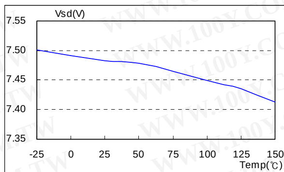
Figure 8. Shutdown Feedback Voltage vs. Temp.
