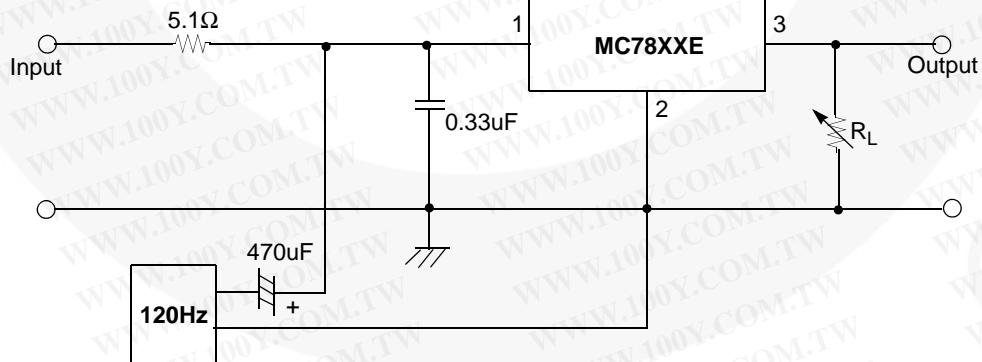
Figure 8. Ripple Rejection
