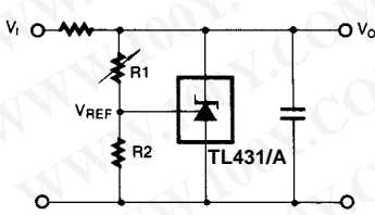
Figure 10. Shunt Regulator
