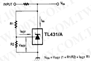
Figure 2. Test Circuit for V_{KA} \geq V_{REF}
