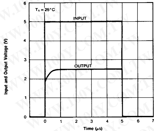
Figure 6. Pulse Response
