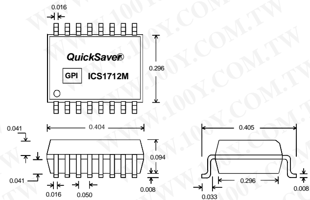
16-Pin SOIC Package (300 mil)
