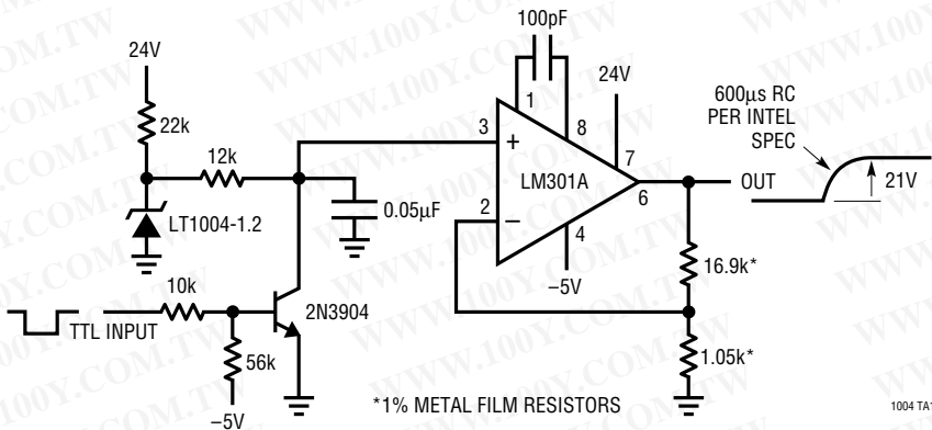
VPP Generator for Eproms — No Trim Required
