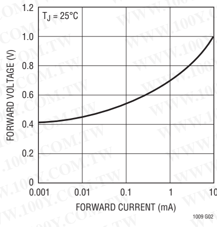
Forward Characteristics
