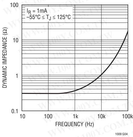
Dynamic Impedance
