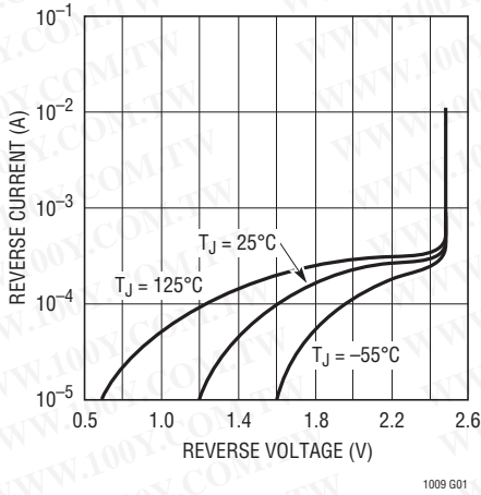
Reverse Characteristics
