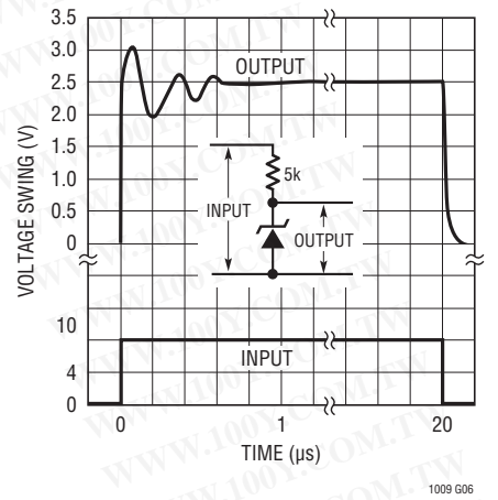
Response Time
