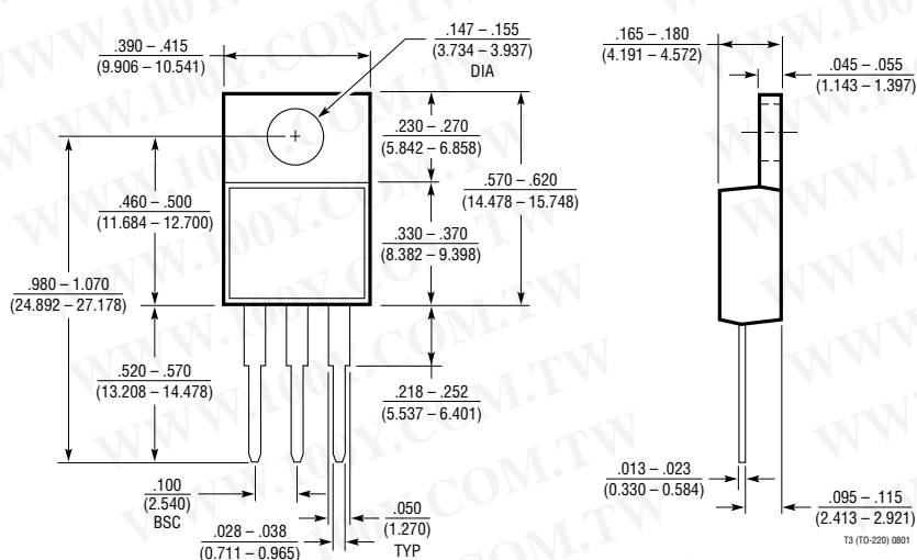
T Package 3-Lead Plastic TO-220 (LTC DWG # 05-08-1420)
