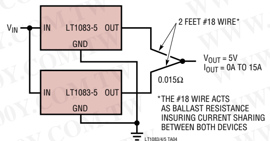
Paralleling Regulators
