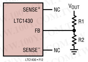
Figure 12. Using External Resistors to Set Output Voltages
