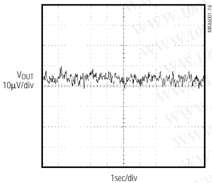
MAX6001 0.1Hz TO 10Hz OUTPUT NOISE
