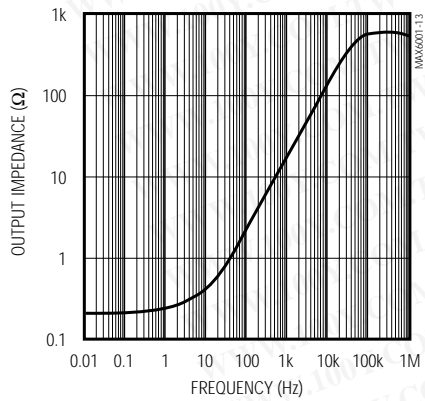
MAX6001 OUTPUT IMPEDANCE vs. FREQUENCY
