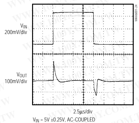
MAX6001 LINE-TRANSIENT RESPONSE
