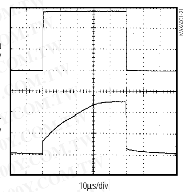
MAX6005 TURN-ON TRANSIENT
