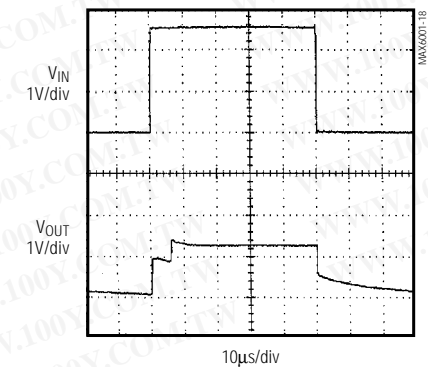
MAX6001 TURN-ON TRANSIENT
