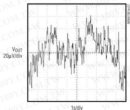
MAX6195 0.1Hz TO 10Hz OUTPUT NOISE
