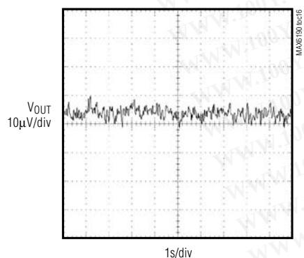
MAX6190 0.1Hz TO 10Hz OUTPUT NOISE
