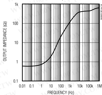
MAX6195 OUTPUT IMPEDANCE vs. FREQUENCY
