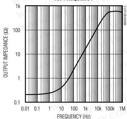
MAX6190 OUTPUT IMPEDANCE vs. FREQUENCY
