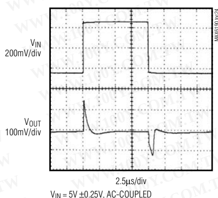
MAX6190 LINE-TRANSIENT RESPONSE
