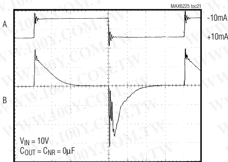
LOAD-TRANSIENT RESPONSE
