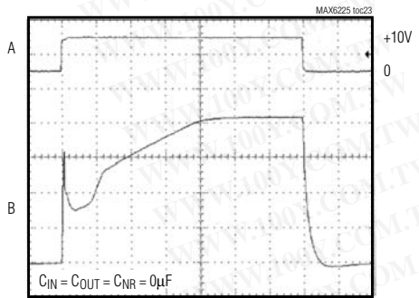
TURN-ON AND TURN-OFF TRANSIENT RESPONSE
