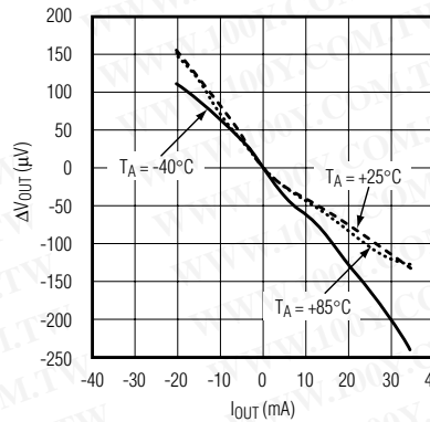
MAX6225 CHANGE IN OUTPUT VOLTAGE vs. OUTPUT CURRENT
