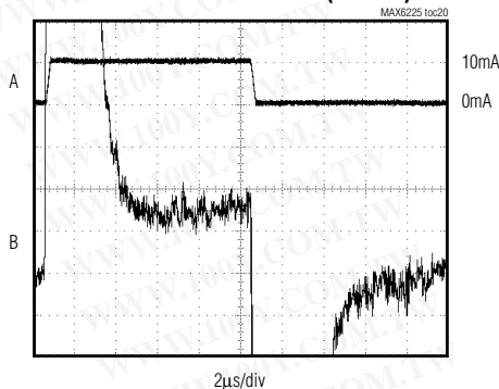
LOAD-TRANSIENT RESPONSE (SINKING)
