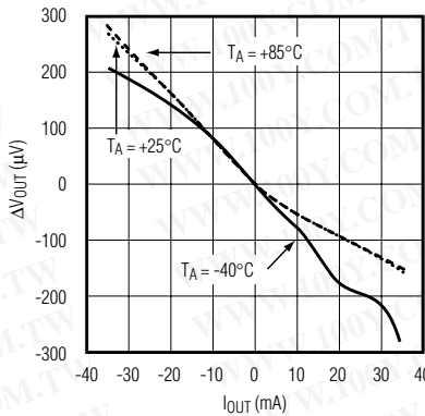
MAX6241 CHANGE IN OUTPUT VOLTAGE vs. OUTPUT CURRENT
