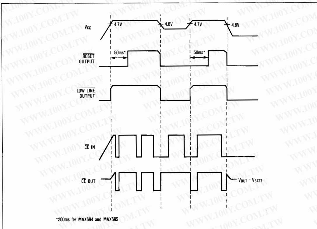
Figure 6. Reset Timing
