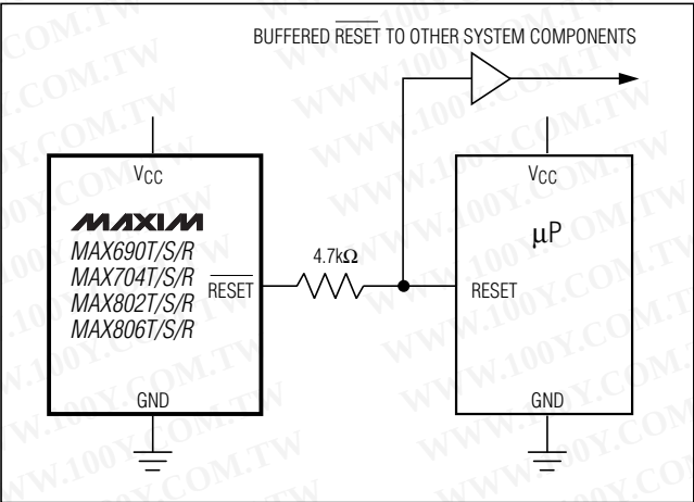
Figure 6. Interfacing to μPs with Bidirectional Reset I/O
