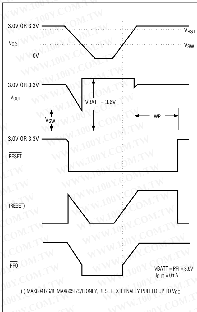
Figure 2. Timing Diagram
