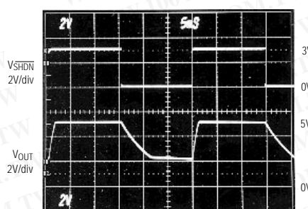
START-UP DELAY
