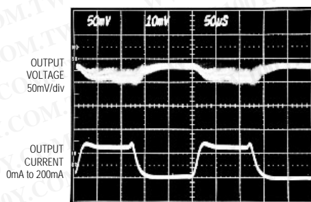
LOAD-TRANSIENT RESPONSE
