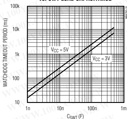
WATCHDOG TIMEOUT PERIOD vs. SWT LOAD CAPACITANCE
