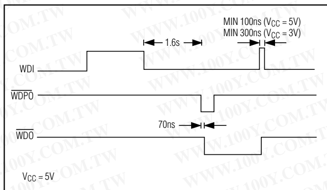
Figure 7. WDI, WDO, and WDPO Timing Diagram
