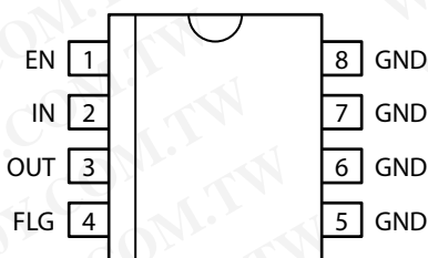
MIC39101-x.x Fixed SOIC-8 (M)
