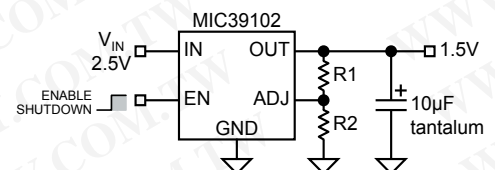
1.5V/1A Adjustable Regulator
