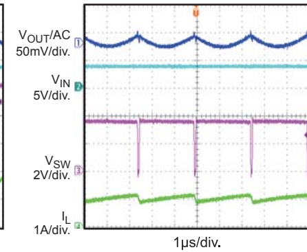
Steady State V IN =3.6V, V OUT =3.3V, I OUT =1A, AAM
