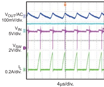
Steady State V IN =3.6V, V OUT =3.3V, I OUT =0.05A, AAM
