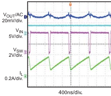
Steady State V IN =3.6V, V OUT =3.3V, I OUT =0.25A, AAM
