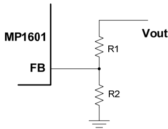
Figure 10: Feedback Network
