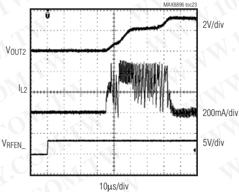
OUT2 STARTUP WAVEFORM
