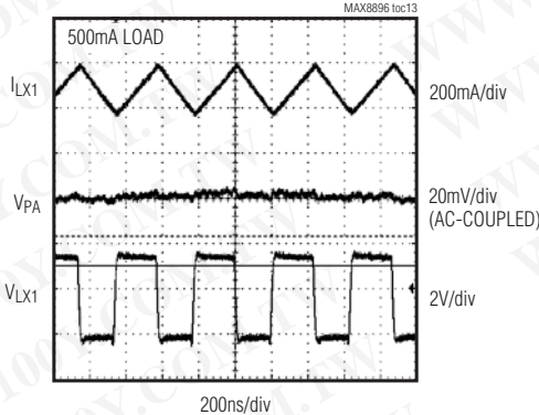
OUT1 HEAVY-LOAD SWITCHING WAVEFORMS
