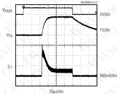
OUT1 STARTUP AND SHUTDOWN
