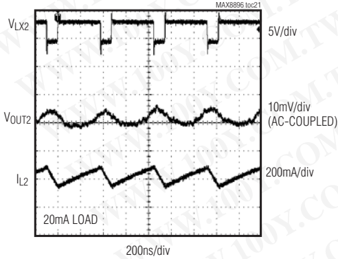
OUT2 LIGHT-LOAD SWITCHING WAVEFORMS
