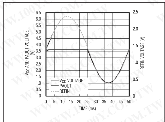
Figure 2. Automatic Bypass
