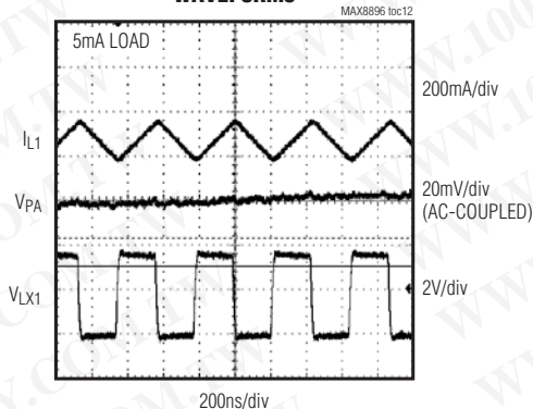
OUT1 LIGHT-LOAD SWITCHING WAVEFORMS
