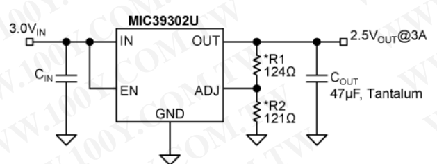
MIC39302 Adjustable Output Application
