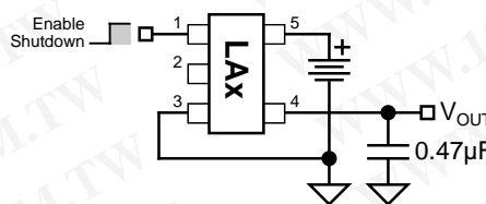
Regulator Circuit
