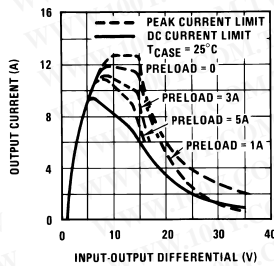
Current Limit
