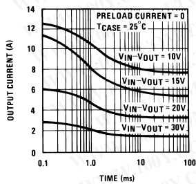
Current Limit
