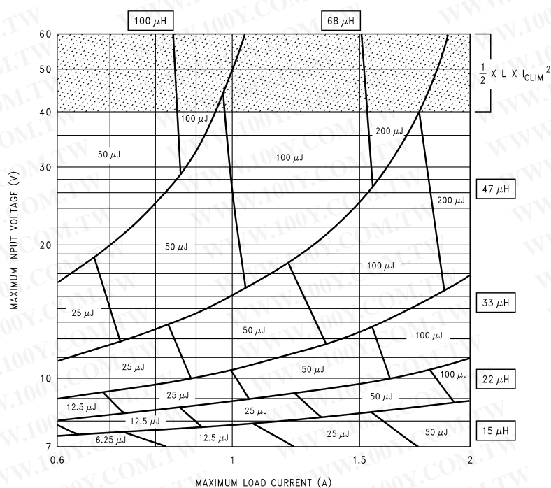
FIGURE 3. LM2592HV-5.0
