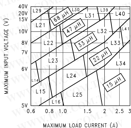
FIGURE 4. LM2596-3.3
