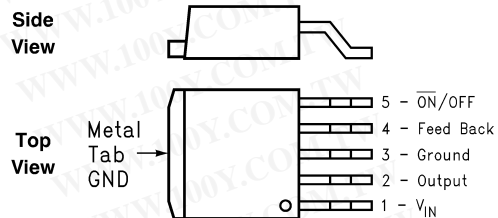
Surface Mount Package 5-Lead TO-263 (S)
