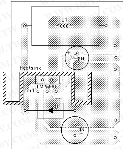
Component Side
