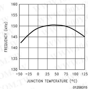
Switching Frequency
