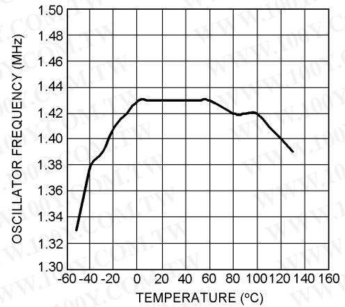
Oscillator Frequency vs Ambient Temperature V_{IN} = 5V
