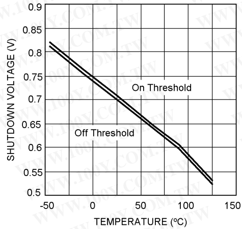
V_{SHUTDOWN} vs Ambient Temperature V_{IN} = 5\text{V}
