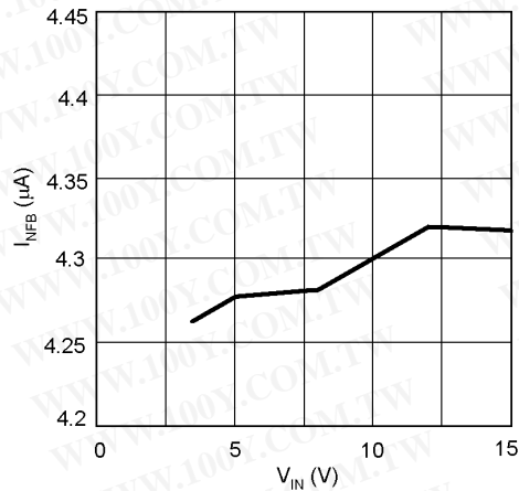
I_{NFB} vs V_{IN} T_A = 25^\circ\text{C} , V_{OUT} = -5\text{V}
