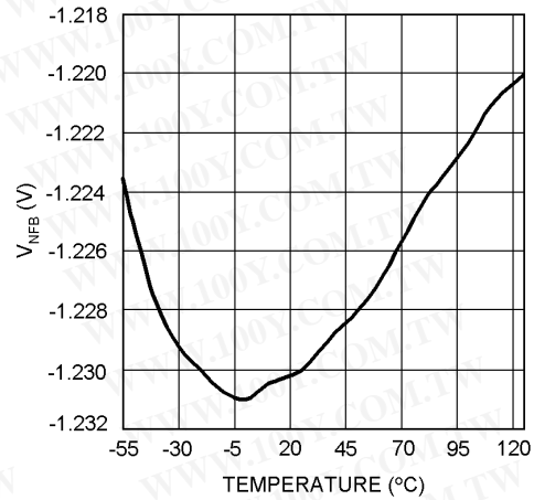
V_{NFB} vs Ambient Temperature V_{IN} = 5\text{V}
