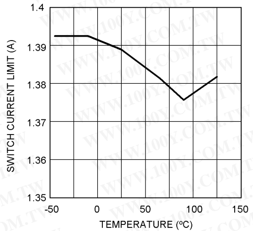
Switch Current Limit vs Ambient Temperature V_{IN} = 5V
