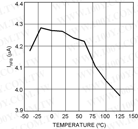
I_{NFB} vs Ambient Temperature V_{IN} = 3.5\text{V} , V_{OUT} = -5\text{V}
