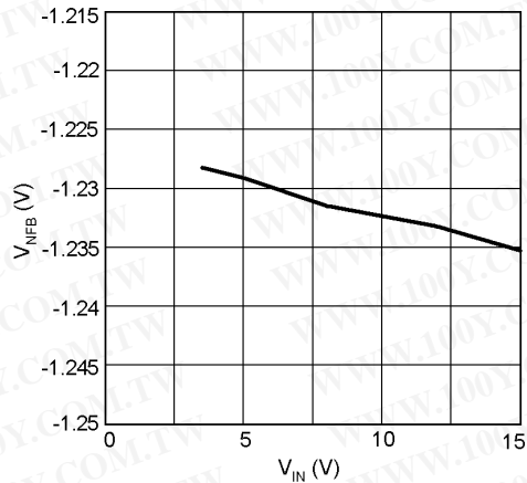
V_{NFB} vs V_{IN} T_A = 25^\circ\text{C} , V_{OUT} = -5\text{V}
