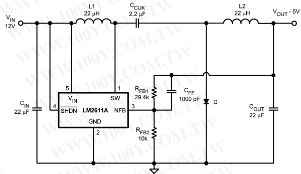
12V to -5V Inverting Converter
