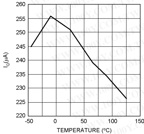
I_Q vs Ambient Temperature (No Load)
