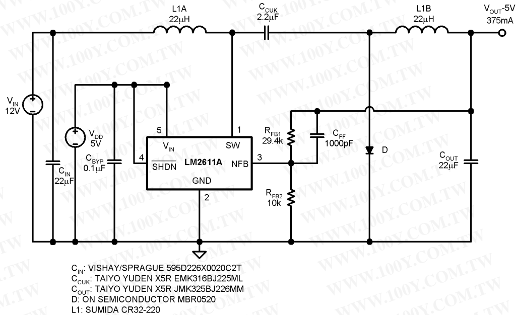
FIGURE 12. LM2611 Operating with Separate Power and Biasing Supplies
