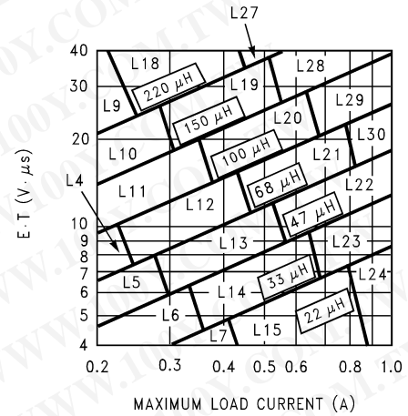
FIGURE 7. LM2672-ADJ
