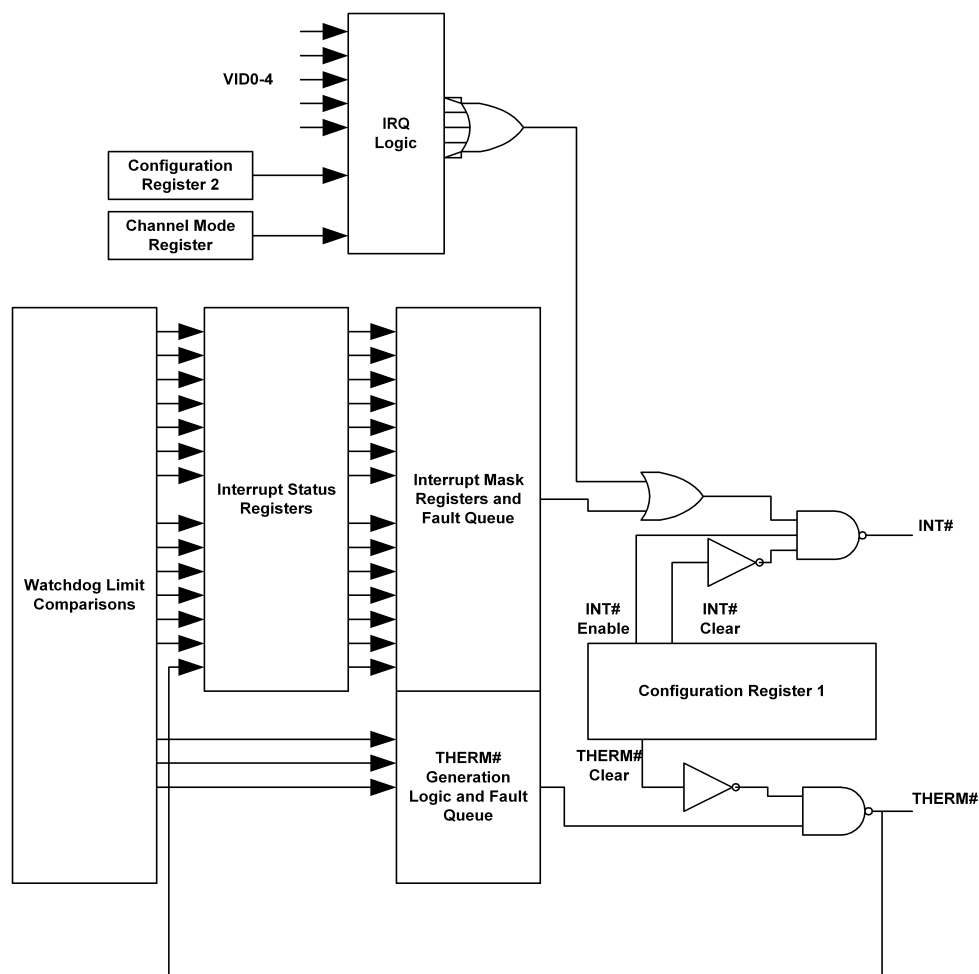
Figure 13. Interrupt Structure
