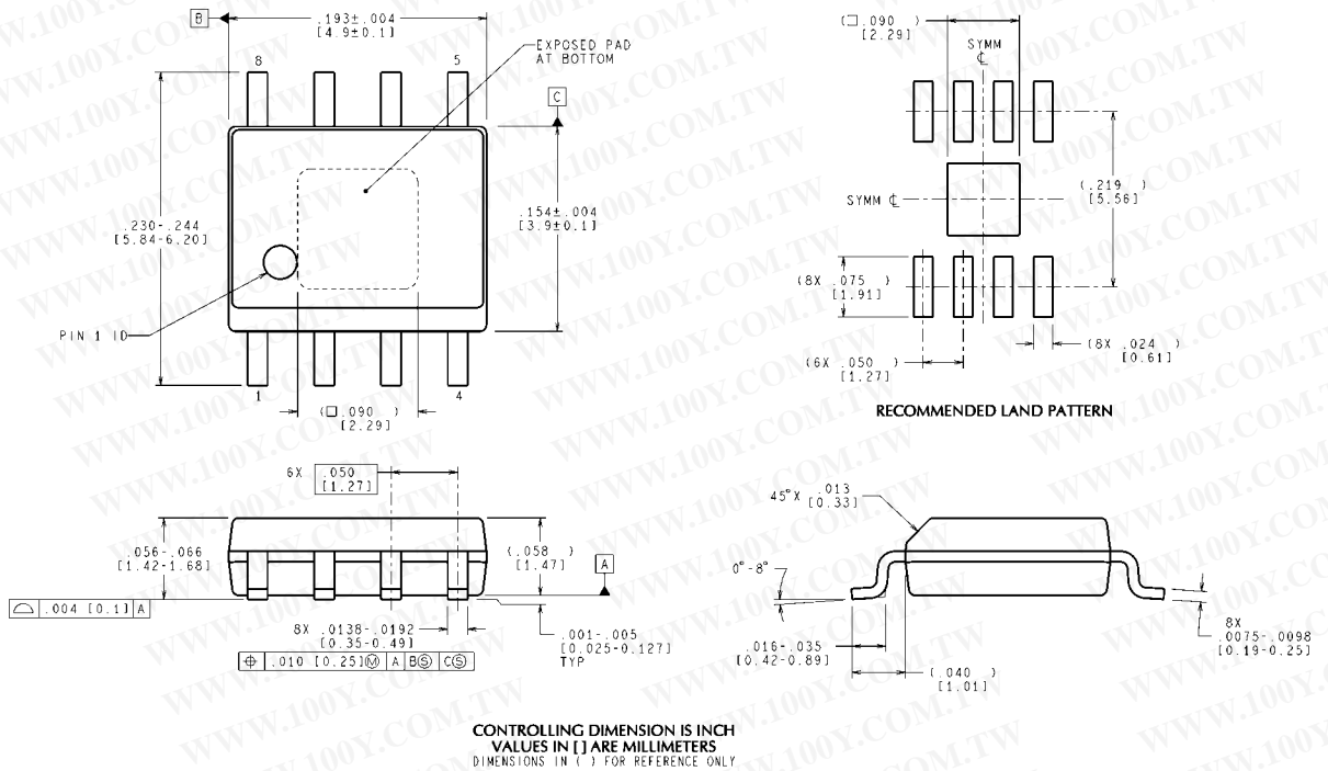
PSOP, 8 Lead, Molded, 0.050in Pitch, Surface Mount NS Package Number MRA08A
