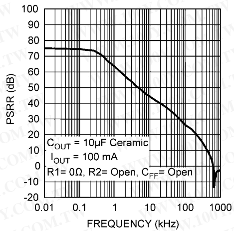
PSRR, I_{OUT} = 100 mA V_{OUT} = V_{ADJ} , C_{OUT} = 10 \mu F Ceramic
