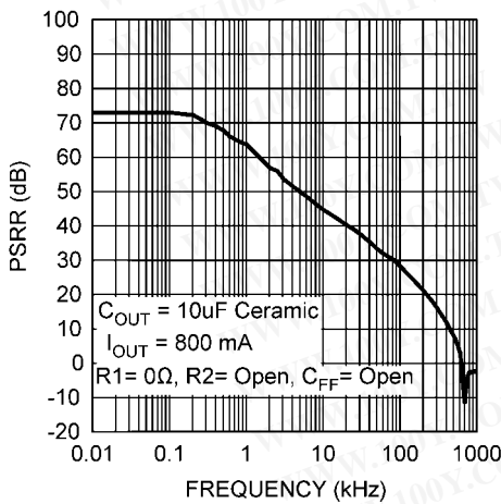
PSRR, I_{OUT} = 800 mA V_{OUT} = V_{ADJ} , C_{OUT} = 10 \mu F Ceramic
