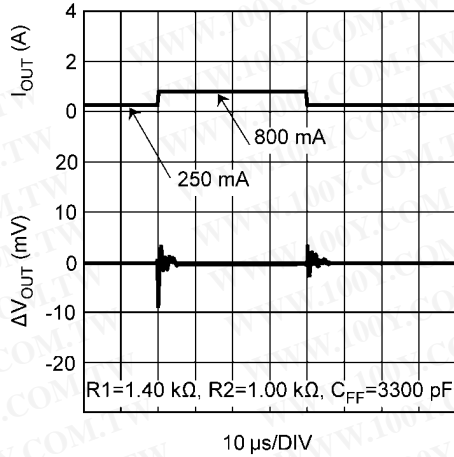
Load Transient, 250 mA to 800 mA V_{OUT} = 1.20V , C_{OUT} = 10 \mu F Ceramic
