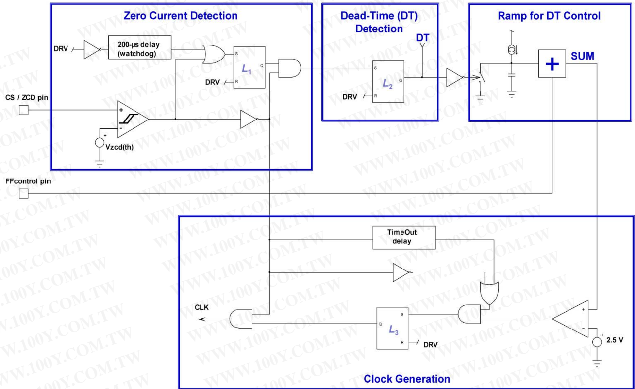
Figure 62. CCFF Practical Implementation
