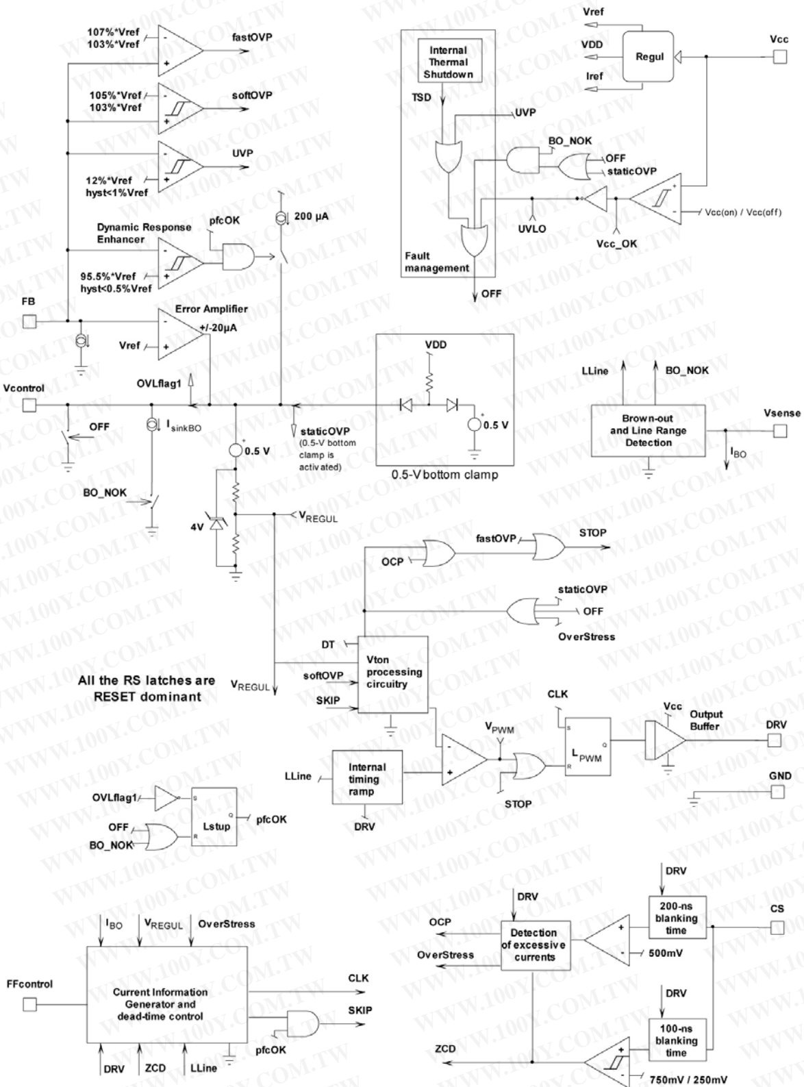
Figure 2. Block Diagram
