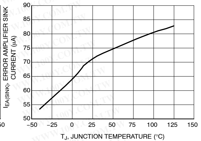
Figure 11. Error Amplifier Sink Current vs. Junction Temperature
