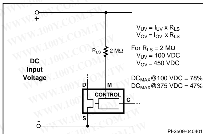
Figure 14. Line Sensing for Under-Voltage, Overvoltage and Maximum Duty Cycle Reduction.
