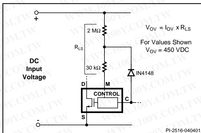
Figure 16. Line Sensing for Overvoltage Only (Under-Voltage Disabled).
