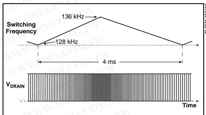
Figure 6. Switching Frequency Jitter.
