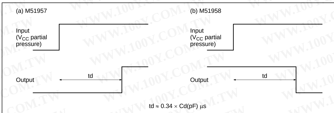
Figure 4 Operating Waveform
