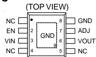
SOP-8 (Exposed Pad)
