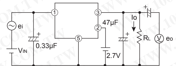
Fig.2 Test Circuit for Ripple Rejection
