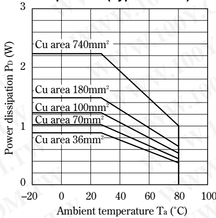
Fig.17 Rower Dissipation vs. Ambient Temperature (Typical Value)
