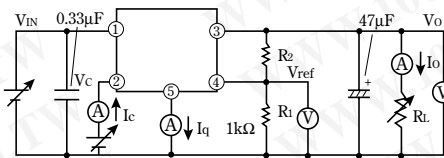
Fig. 1 Test Circuit
