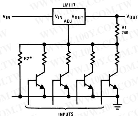
Figure 45. Digitally Selected Outputs
