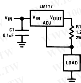
Figure 31. 1A Current Regulator
