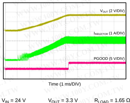
Figure 92. Startup Into Full Load with Internal Soft-Start Rate
