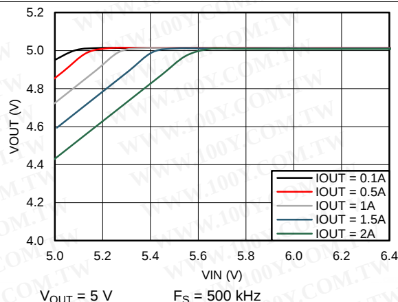
Figure 56. Drop-Out Curve
