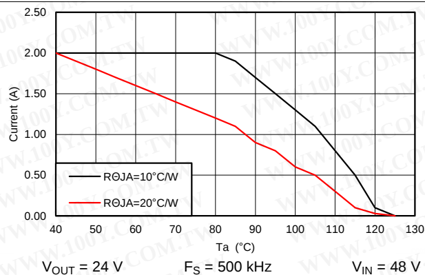
Figure 82. Derating Curve
