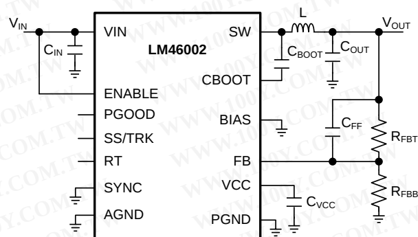
Figure 45. LM46002 Basic Schematic for V_{OUT} < 3.3 V, t-Tie BIAS to Ground
