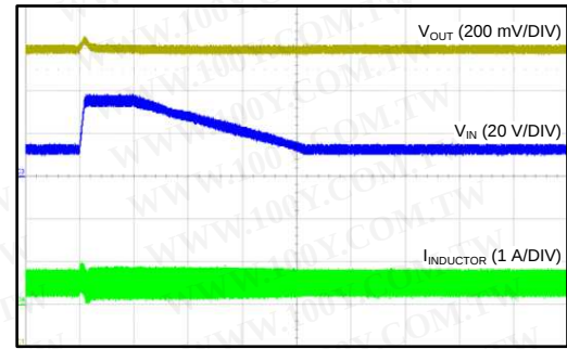
Time (500 \mu\text{s} /DIV) V_{OUT} = 3.3\text{ V} F_S = 500\text{ kHz} I_{OUT} = 0.5\text{ A}
