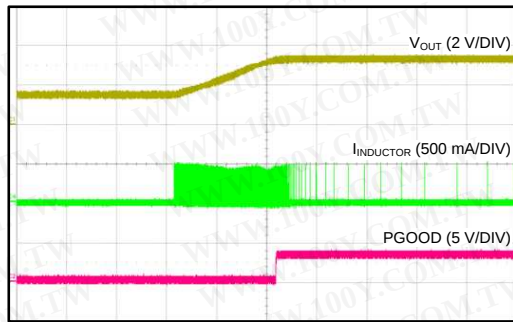
Time (1 ms/DIV) V_{IN} = 24\text{ V} V_{OUT} = 3.3\text{ V} R_{LOAD} = \text{Open}
