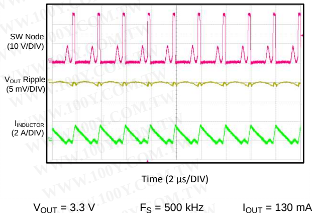
Figure 90. Switching Waveform in DCM Operation
