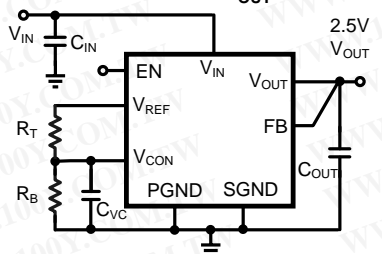
Schematic V_{OUT} = 2.5V
