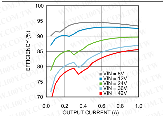
Figure 1. Efficiency V_{OUT} = 5\text{ V} , T_A = 25^\circ\text{C}
