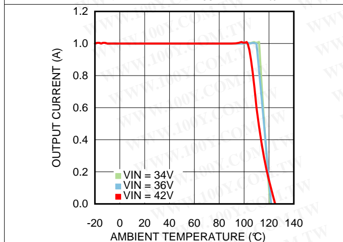
Figure 29. Thermal Derating V_{OUT} = 30\text{ V} , R_{\theta JA} = 16^\circ\text{C/W}
