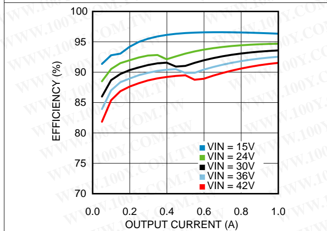
Figure 3. Efficiency V_{OUT} = 12\text{ V} , T_A = 25^\circ\text{C}
