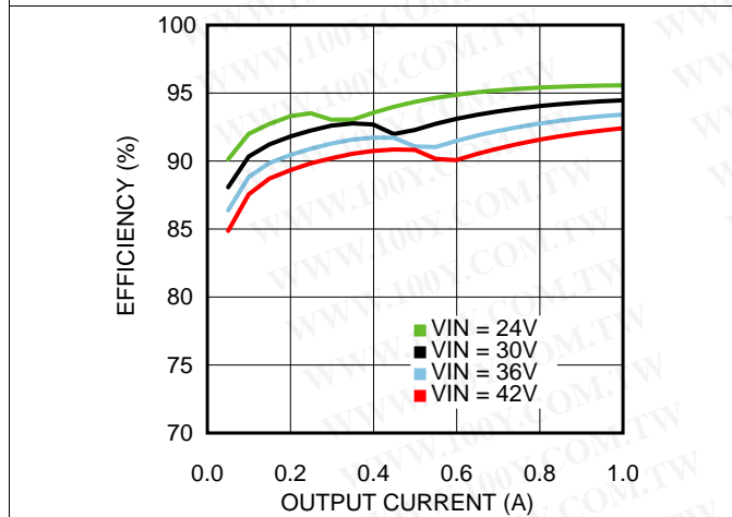
Figure 5. Efficiency V_{OUT} = 15\text{ V} , T_A = 25^\circ\text{C}
