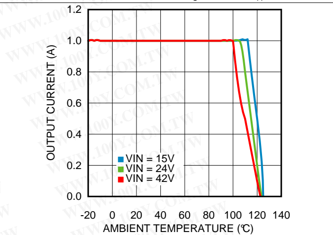
Figure 26. Thermal Derating V_{OUT} = 12\text{ V} , R_{\theta JA} = 20^\circ\text{C/W}
