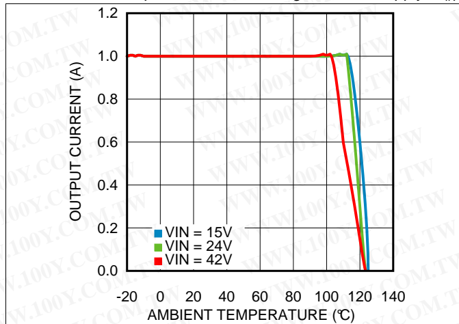
Figure 25. Thermal Derating V_{OUT} = 12\text{ V} , R_{\theta JA} = 16^\circ\text{C/W}
