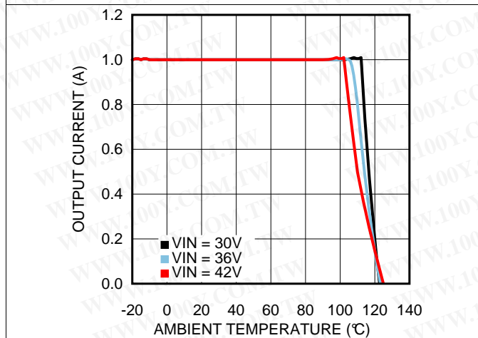
Figure 27. Thermal Derating V_{OUT} = 24\text{ V} , R_{\theta JA} = 16^\circ\text{C/W}
